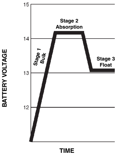
CHARGING PROFILE
